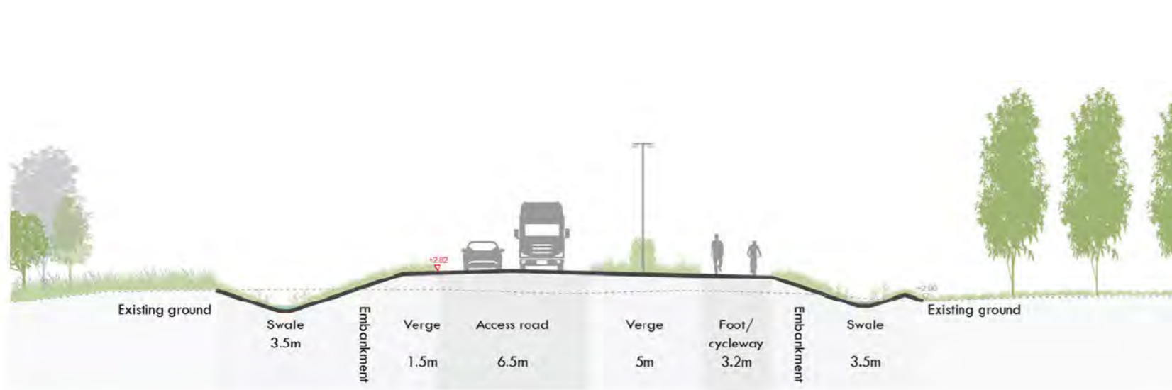
Figure 5.16: Illustrative Road Corridor Sections
