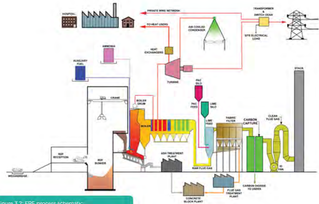
Figure 3.2: ERF process schematic
